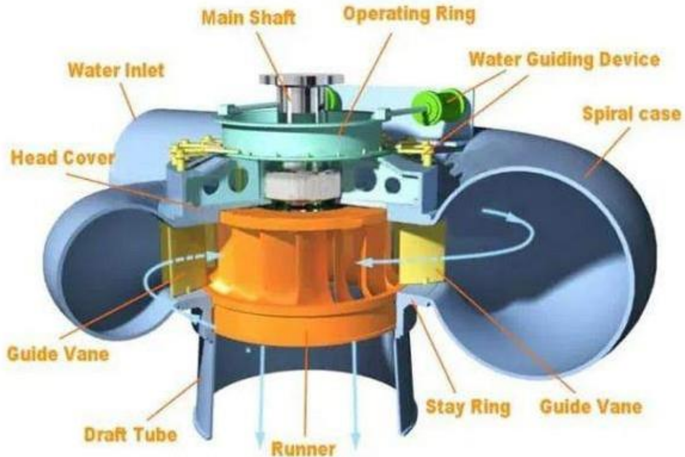
Francis Turbine
