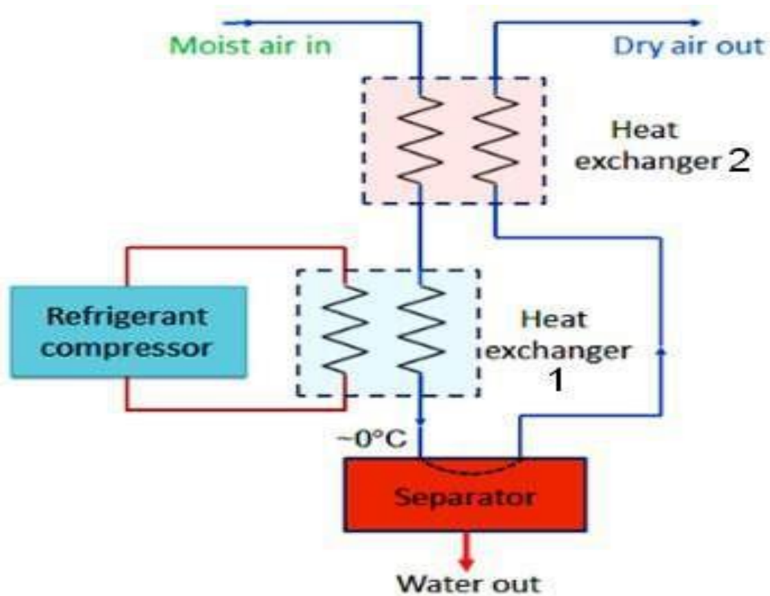
Fig 13 refrigerated dryer
